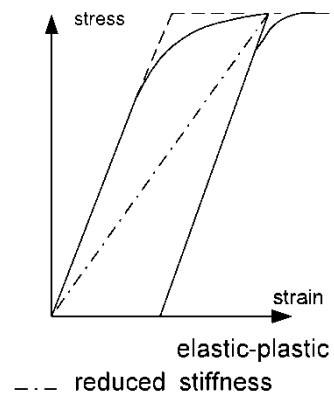
Figure 2.2. Elastic –full plastic behavior
